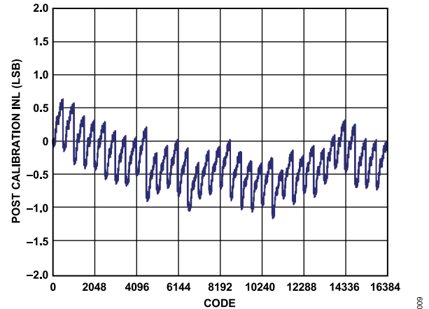
Figure 9. AD9117 Postcalibration INL at 1.8 V, 8 mA (DVDD = 1.8 V)
