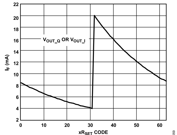
Figure 99. Effect of xR_{SET} Code
