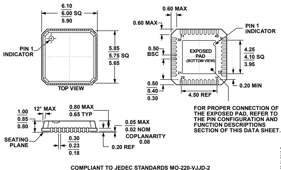
Figure 112. 40-Lead Lead Frame Chip Scale Package [LFCSP] 6 mm x 6 mm and 0.85 mm Package Height (CP-40-1) Dimensions shown in millimeters
