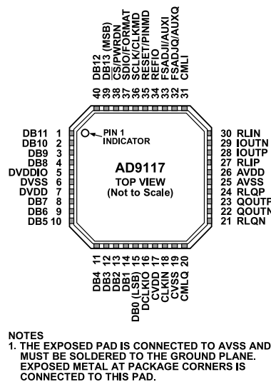
Figure 5. AD9117 Pin Configuration
