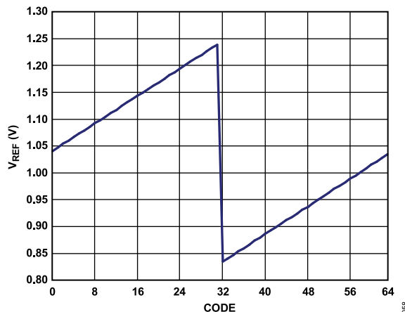
Figure 98. Typical V_{REF} Voltage vs. Code
