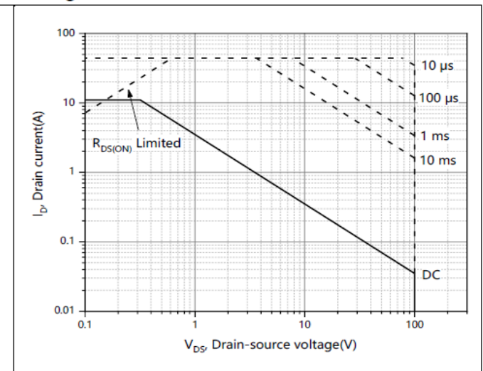
Figure 10, Safe operation area T_C = 25\text{ }^{\circ}\text{C}
