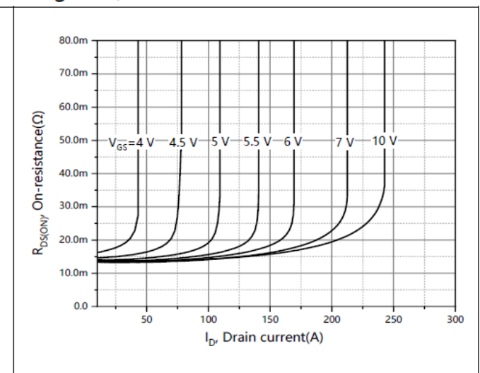
Figure 8, Drain-source on-state resistance
