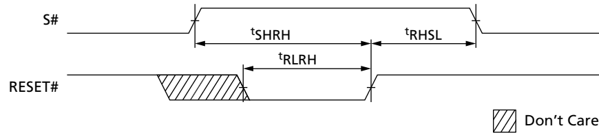
Figure 51: Reset Enable and Reset Memory Timing
