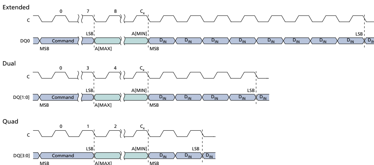
Figure 44: PROGRAM OTP Command Timing
