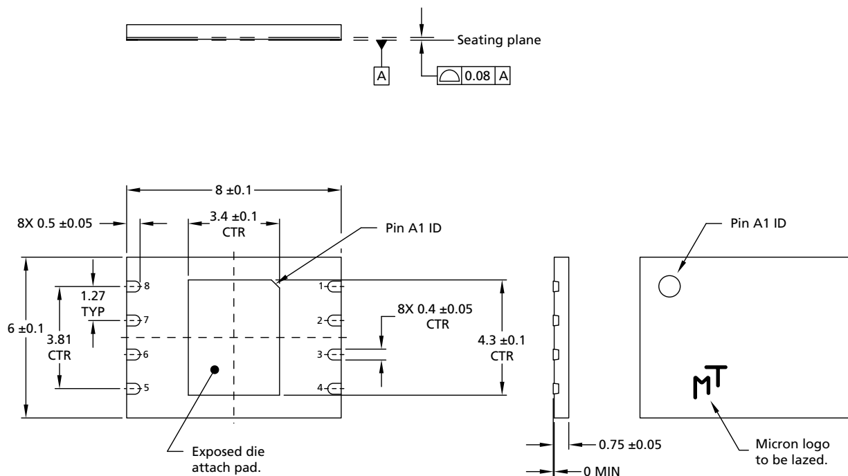
Figure 12: W-PDFN-8 (MLP8) – 8mm x 6mm
