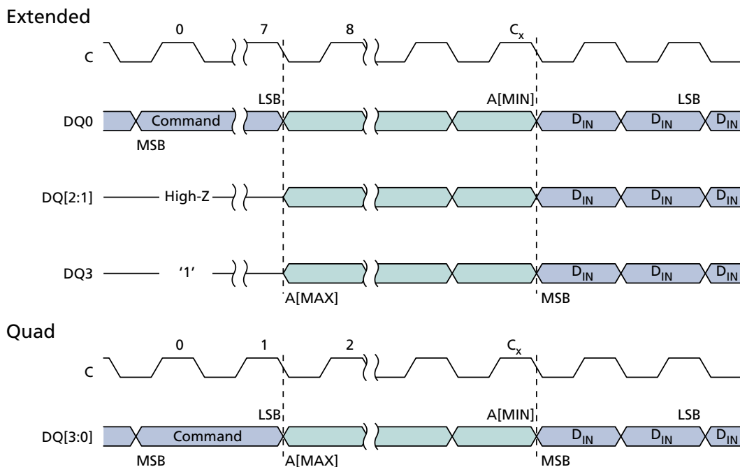
Figure 39: EXTENDED QUAD INPUT FAST PROGRAM Command
