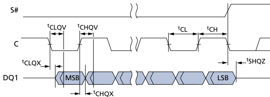
Figure 57: Output Timing for DTR
