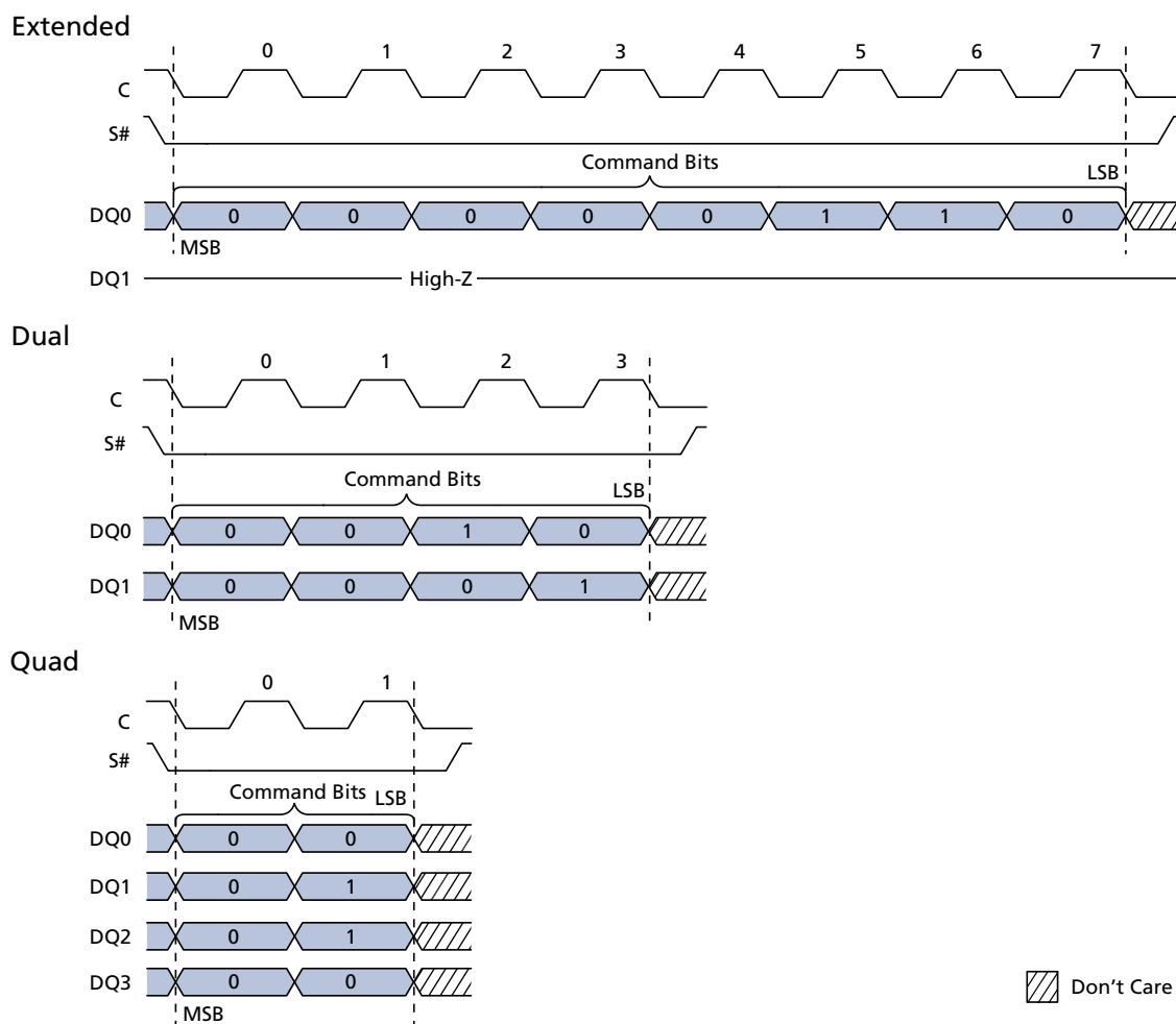
Figure 31: WRITE ENABLE and WRITE DISABLE Timing
