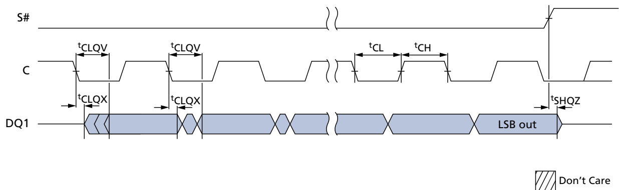
Figure 56: Output Timing for STR
