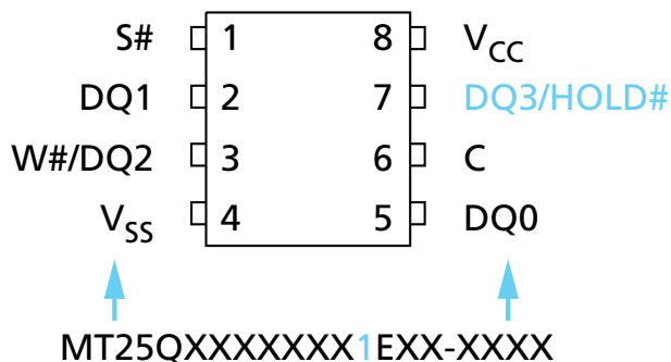
Figure 7: 8-Pin, SOP2 or W-PDFN (Top View)
