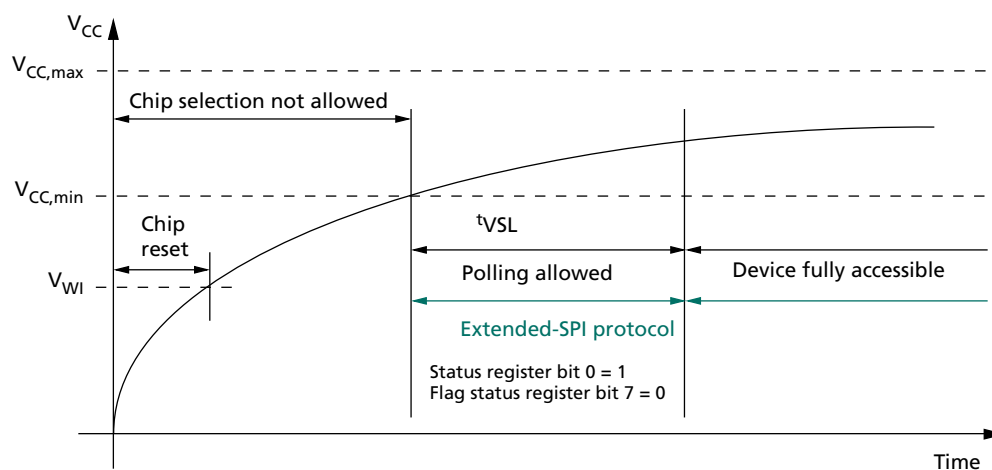
Figure 48: Power-Up Timing
