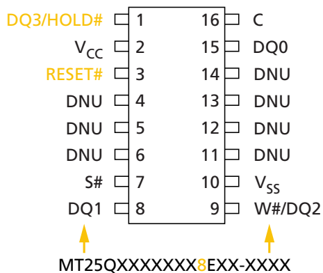
Figure 6: 16-Pin, Plastic Small Outline – SO16 (Top View)
