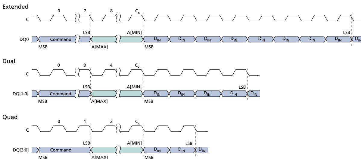
Figure 35: PAGE PROGRAM Command
