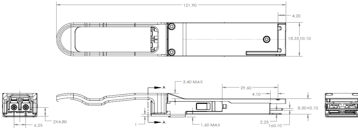
Figure 2 – FTL4C1QE3L mechanical drawing
