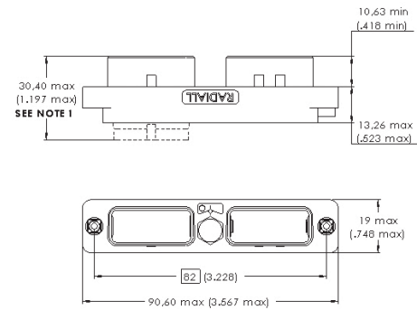
Plug [PB]
