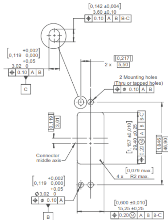
Plug - Shown from the Front Side
