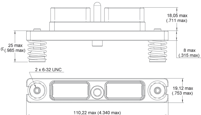
Rear Mount
