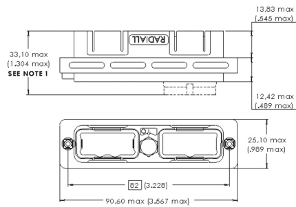
Receptacle [LL]
