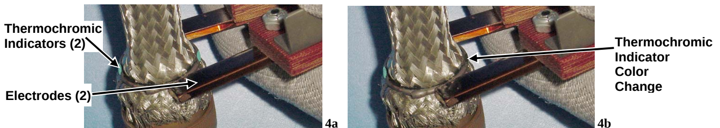
Figure 4. Heating the Ring and Thermochromic Indicator Color Change
