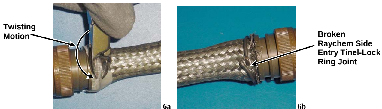
Figure 6. Raychem Side Entry Tinel-Lock Ring Broken
