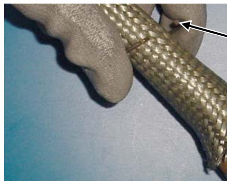
Figure 2. Pressing the Ring together on the Cable Braid
