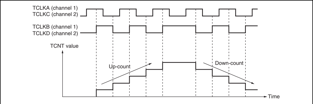
Figure 11.33 Example of Phase Counting Mode 4 Operation
