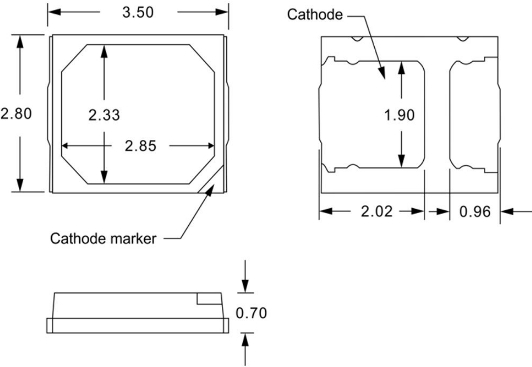
Figure 8. Mechanical dimensions for LUXEON 2835 Commercial
