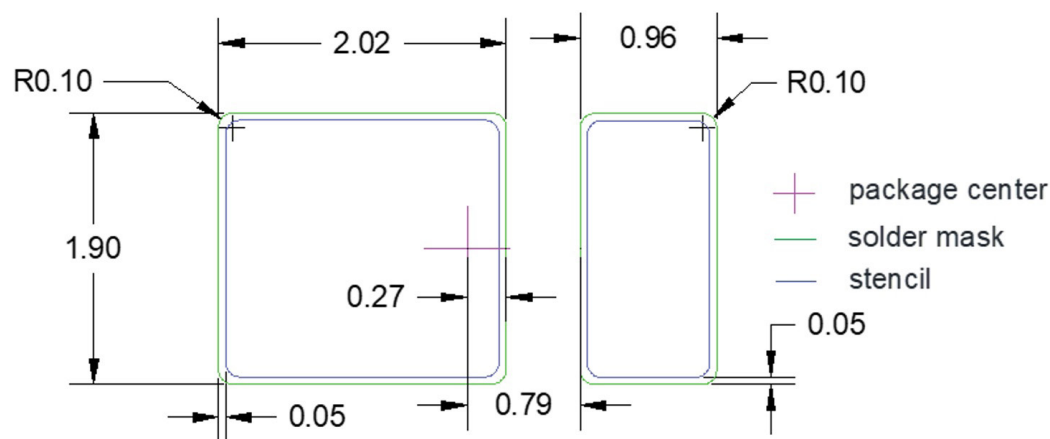
Figure 10. Recommended PCB solder pad layout for LUXEON 2835 Commercial.
