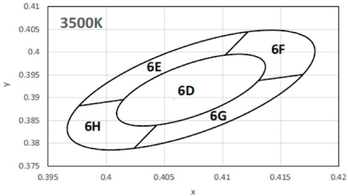
Figure 7d. 1/5 th color bin structure for LUXEON 2835 Commercial 3500K at specified test current and binning temperature of T j =25°C
