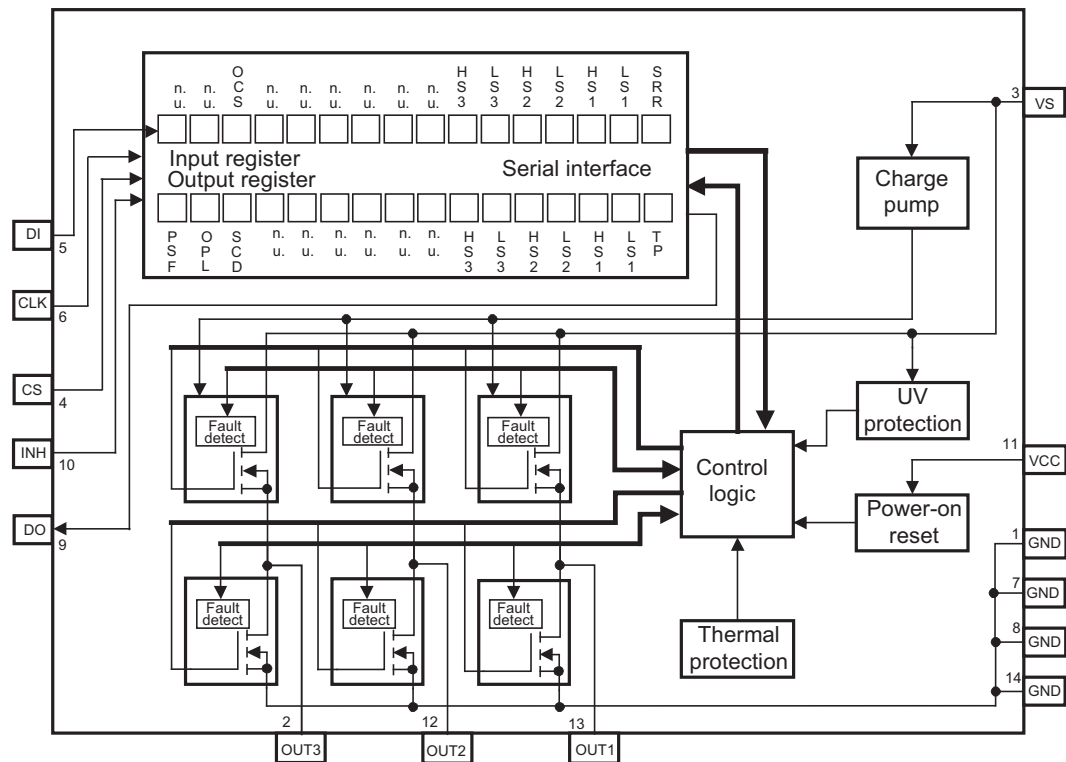
Figure 1-1. Block Diagram
