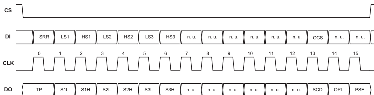
Figure 3-1. Data Transfer
