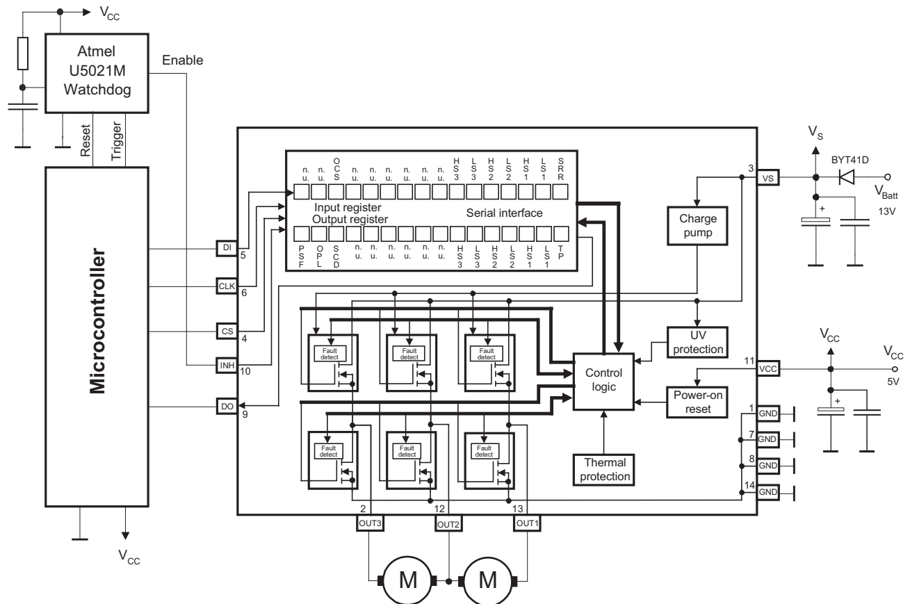
Figure 10-1. Application Circuit
