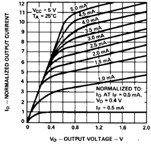
Figure 2 Normalized DC Transfer Characteristics
