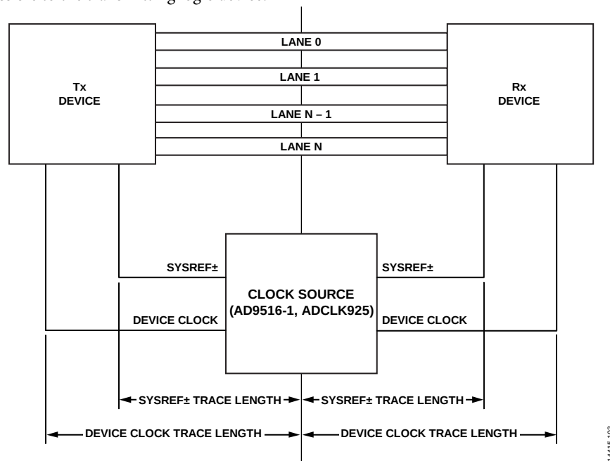
Figure 125. SYSREF± Signal and Device Clock Trace Length
