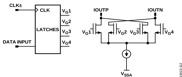
Figure 126. Quad-Switch Architecture
