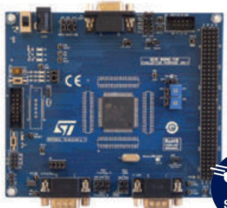
Discovery Kit for the L Line with SPC56EL70L5. order code: SPC56EL70L5DISP
