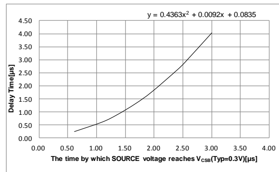
Figure 6B. Delay Time vs the Time by Which the SOURCE Pin Voltage Reaches V_{CSB} (Typ=0.3 V) (BM2P101E)
