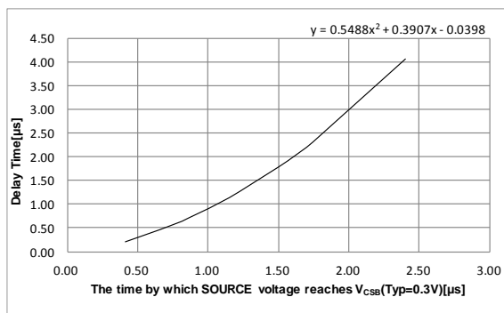
Figure 6C. Delay Time vs the Time by Which the SOURCE pin Voltage Reaches V_{CSB} (Typ=0.3 V) (BM2P131E)
