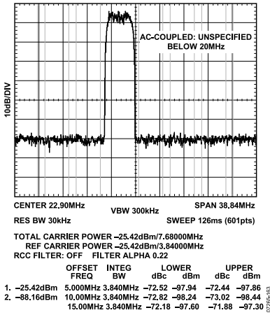
Figure 65. AD9717 One-Carrier ACLR, 3.3 V
