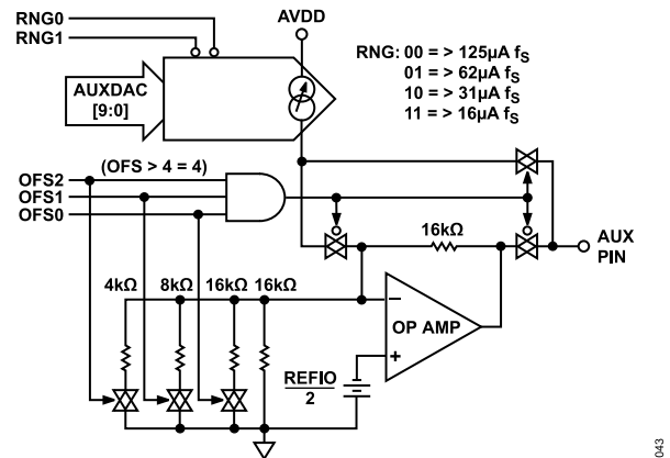
Figure 107. AUXDAC Simplified Circuit Diagram
