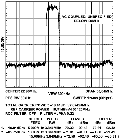
Figure 62. AD9717 One-Carrier ACLR, 1.8 V
