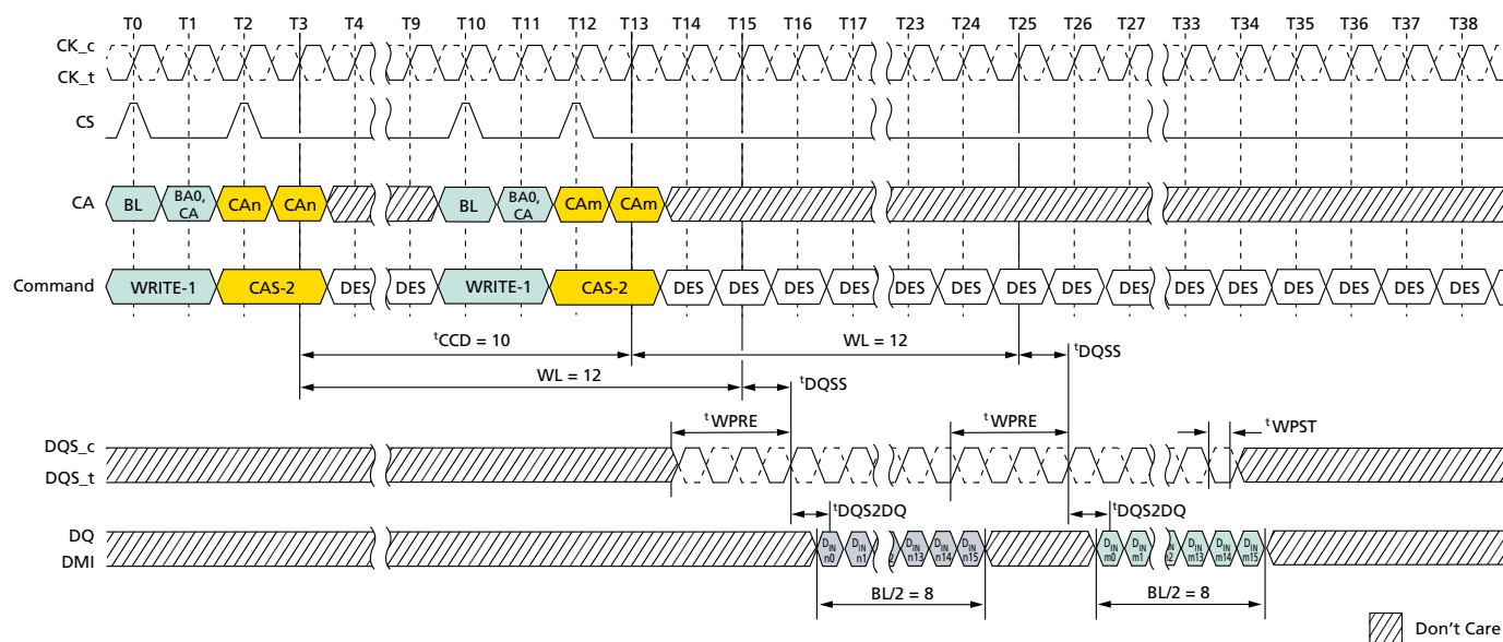
Figure 59: Consecutive WRITE: t_{CCD} = \text{MIN} + 2, 0.5n\text{CK} Postamble
