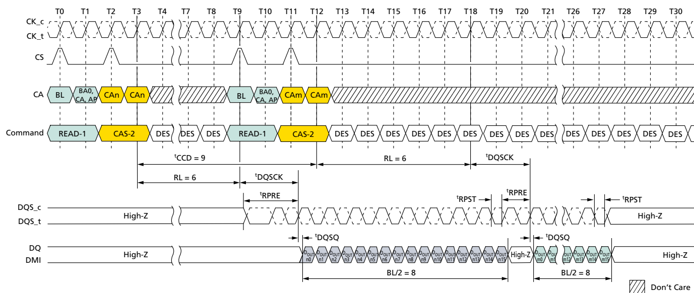
Figure 43: Consecutive READ: t_{CCD} = \text{MIN} + 1 , Preamble = Toggle, 0.5n\text{CK} Postamble
