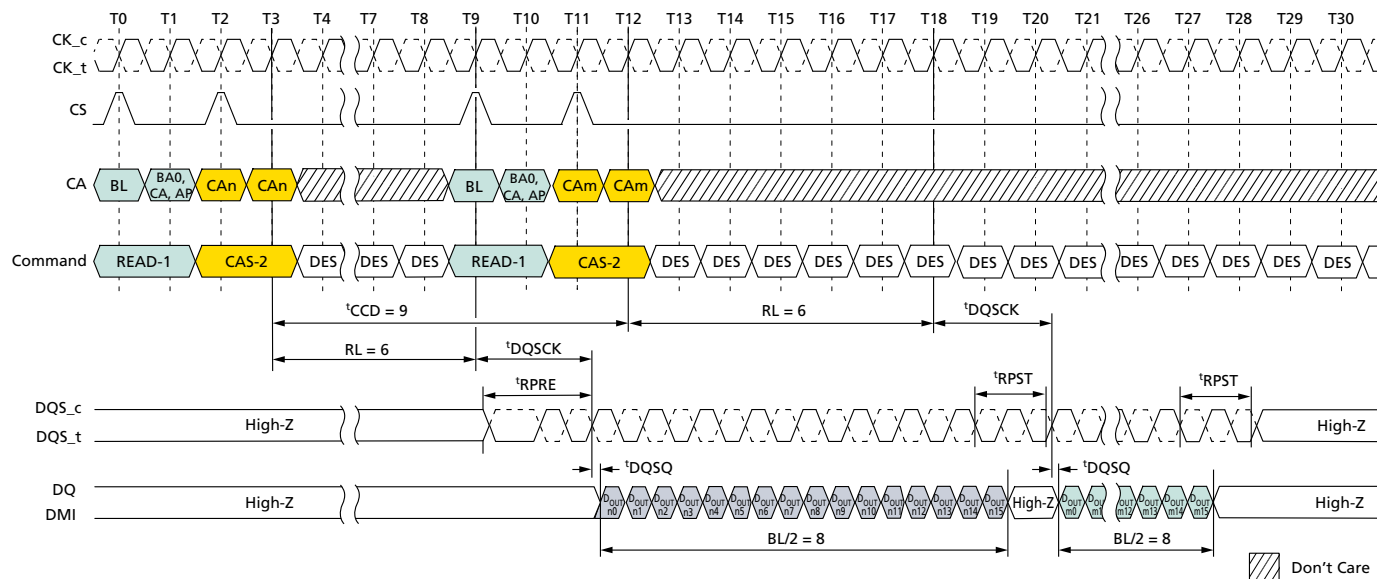
Figure 42: Seamless READ: t_{CCD} = \text{MIN} + 1 , Preamble = Toggle, 1.5n\text{CK} Postamble
