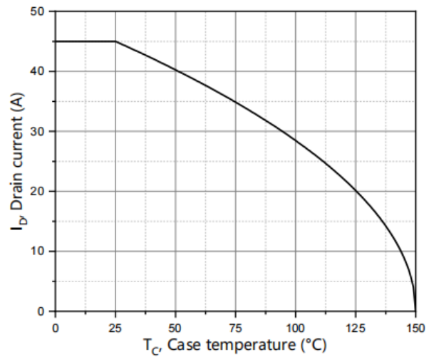
Figure 10. Drain current
