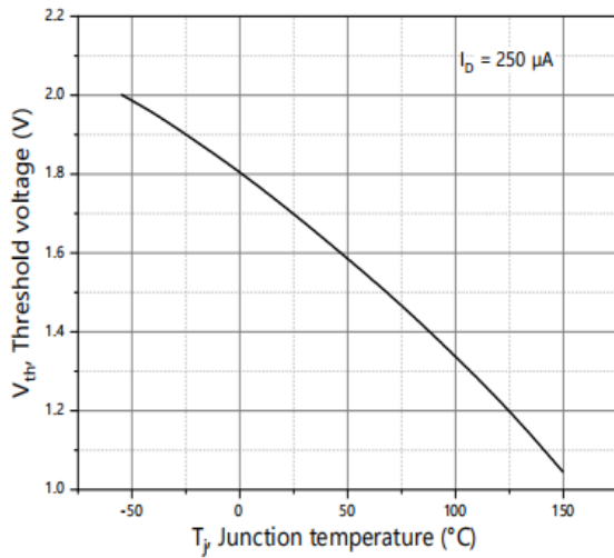
Figure 7. Threshold voltage
