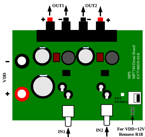
Figure 5—EV7740DN-01B Connection Diagram
