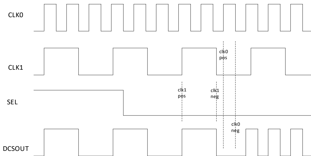
Figure 2.10. DCS Waveforms
