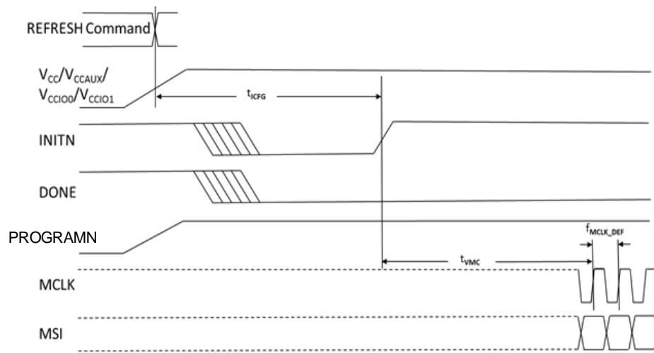
Figure 3.14. Master SPI POR/REFRESH Timing
