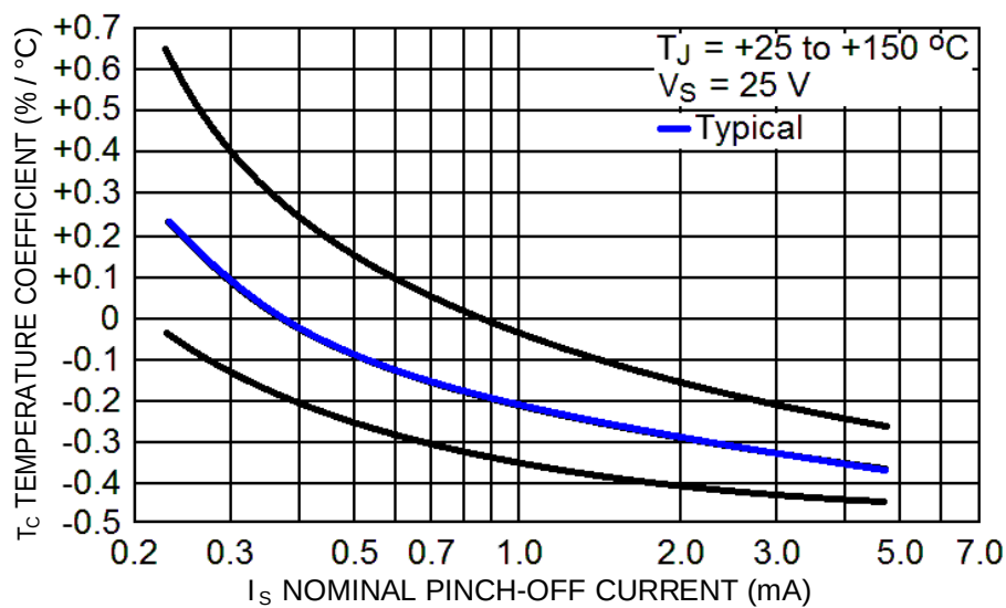
FIGURE 2 – TEMPERATURE COEFFICIENT
