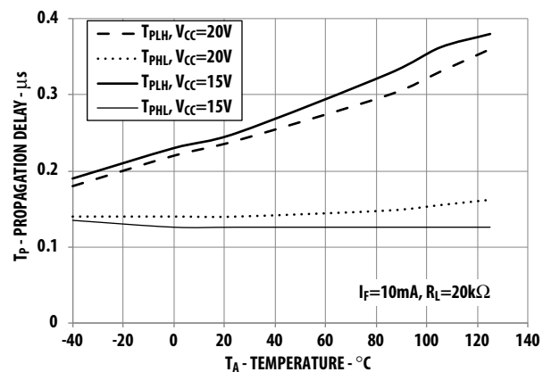
Figure 6 Propagation Delay Time vs Temperature
