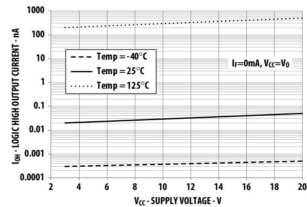
Figure 13 Logic High Output Current vs Supply Voltage
