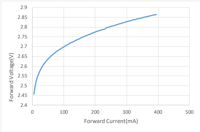
Forward Current vs. Forward Voltage (Tc = 25°C)
