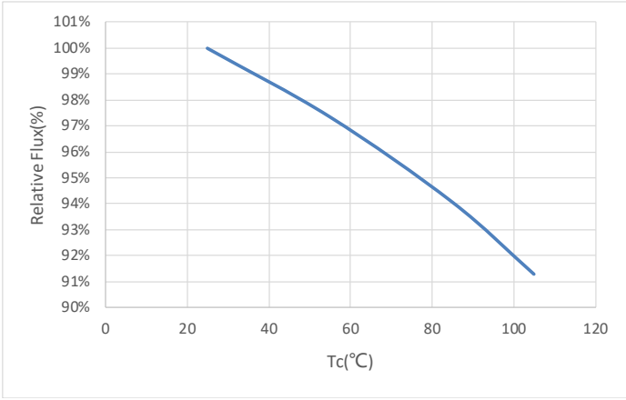
Case Temperature vs. Relative Luminous Flux
