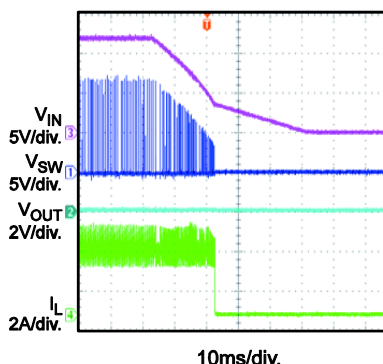
LED+ Short to GND Input Power Off
