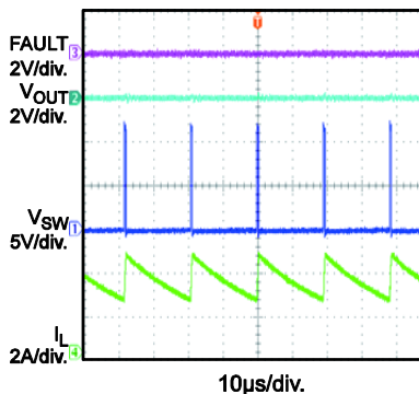
LED+ Short to GND Steady State
