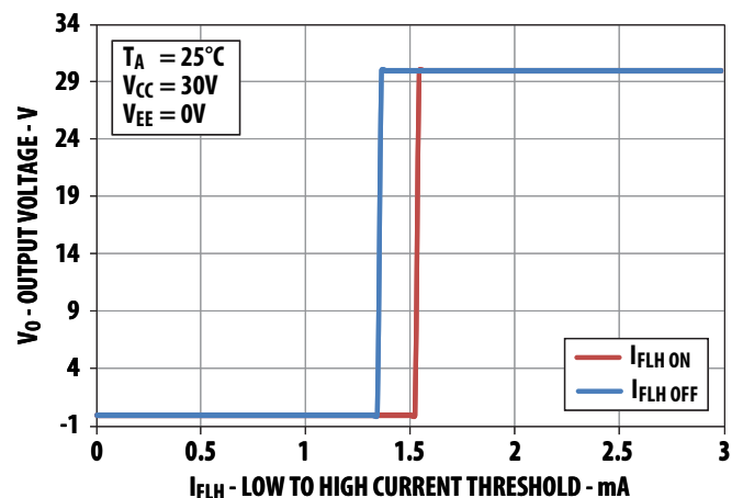
Figure 6 I_{FLH} Hysteresis
