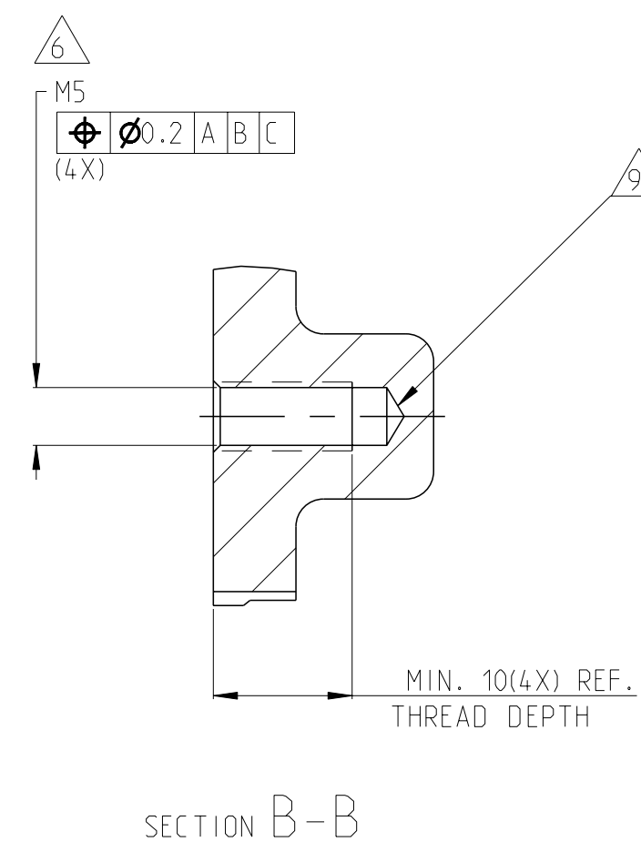
SECTION B-B
