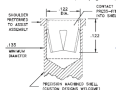
#08 CONTACT FOR .084"-.102" DIAMETER PINS (δ = .011) 6-FINGER (See page 248)
