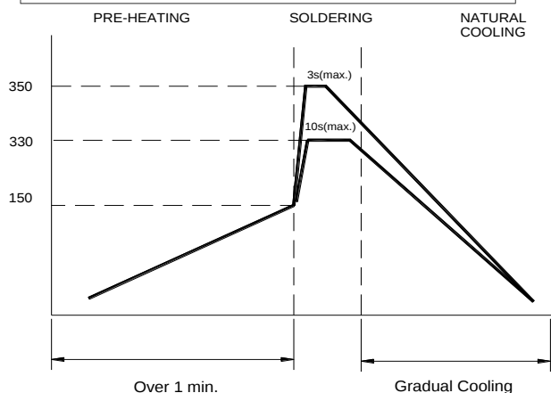
Figure 2. Hand Soldering
