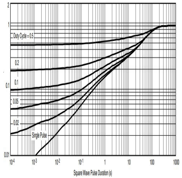
Fig8. Normalized transient thermal impedance
