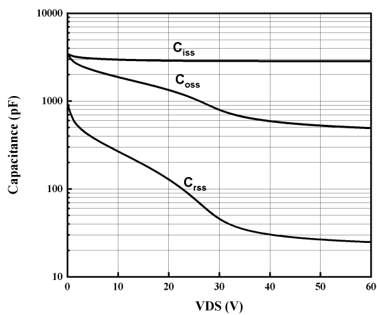
Fig5. Typical Capacitance
