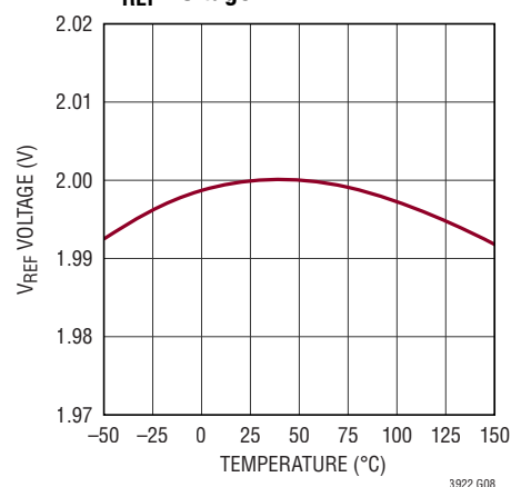
V_{REF} Voltage
