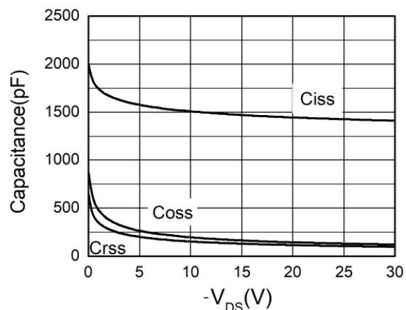
Figure 8. Capacitance
