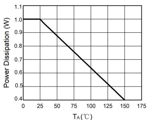
Figure 3. Power Dissipation
