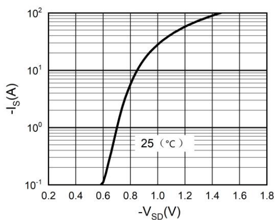
Figure 9. Body-Diode Characteristics
