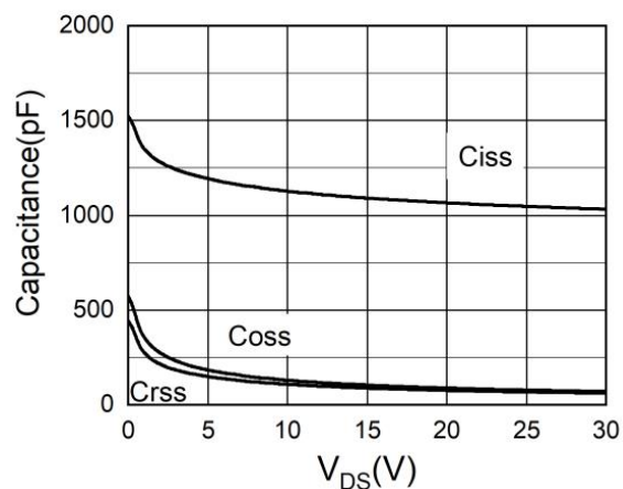
Figure 8. Capacitance
