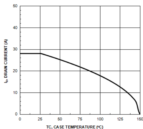
Figure 4. Drain Current
