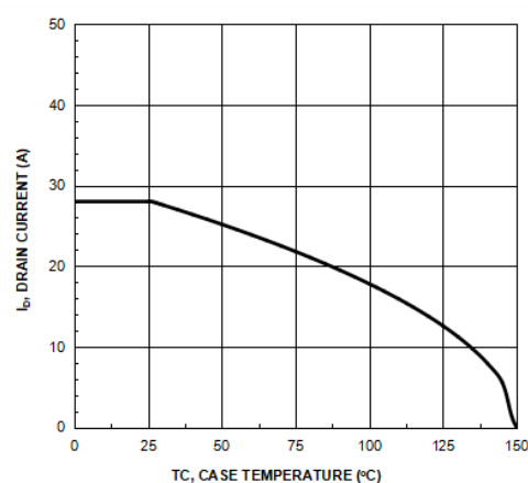
Figure 4. Drain Current
