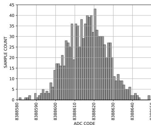
Figure 8. Histogram (Output Data Rate = 2.5 kSPS)
