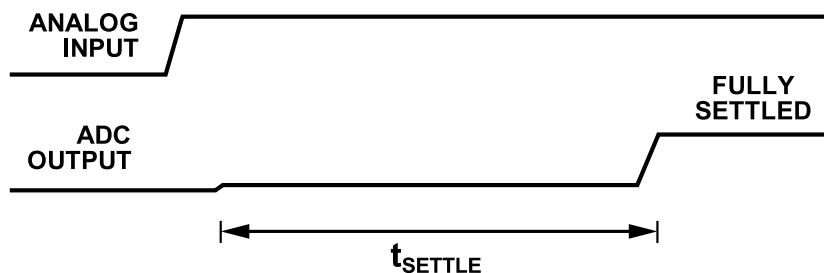
Figure 30. Step Input with Single Cycle Settling
