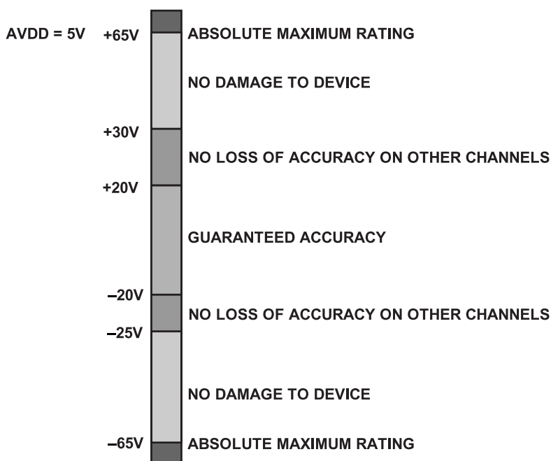
Figure 23. Absolute Input Pin Voltages, AVDD = 5 V
