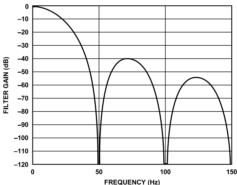
Figure 28. Sinc3 Filter Response
