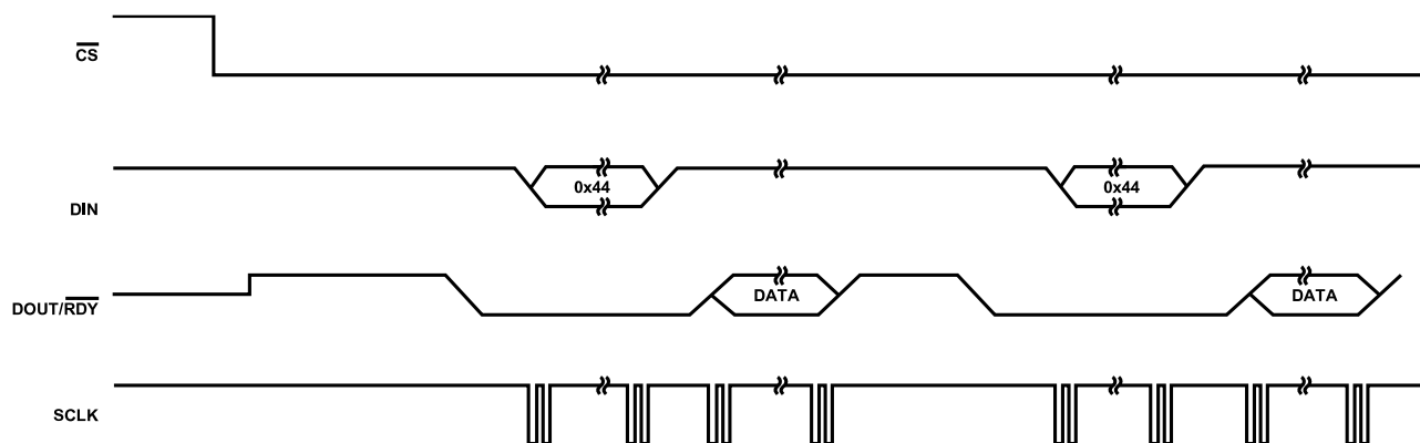
Figure 39. SPI Communication in Continuous Conversion Mode
