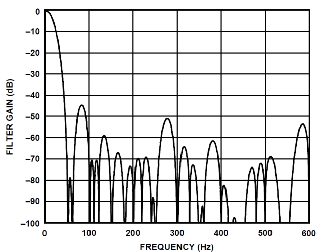
Figure 36. 16.667 SPS ODR, 60 ms Settling Time
