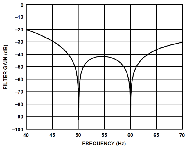
Figure 35. 27.27 SPS ODR, 36.67 ms Settling Time (40 Hz to 70 Hz)
