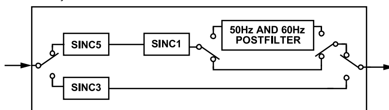
Figure 26. Digital Filter Block Diagram
