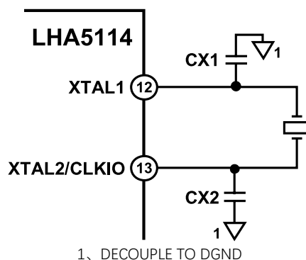
Figure 25. External Crystal Connections
