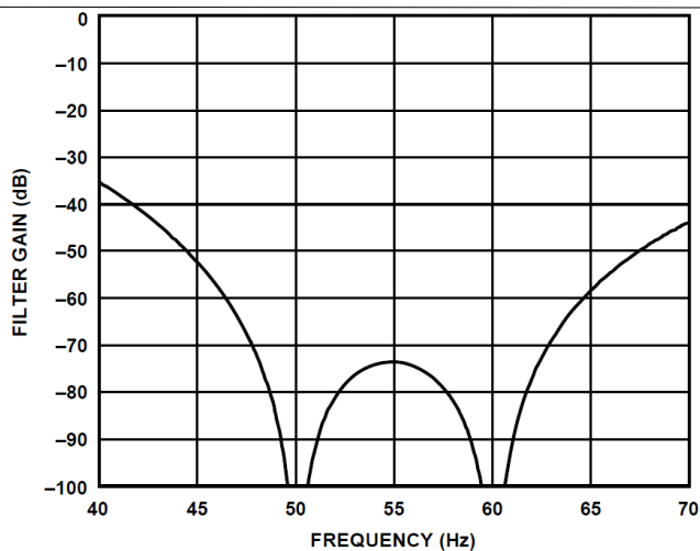
Figure 34. 20 SPS ODR, 50 ms Settling Time (40 Hz to 70 Hz)
