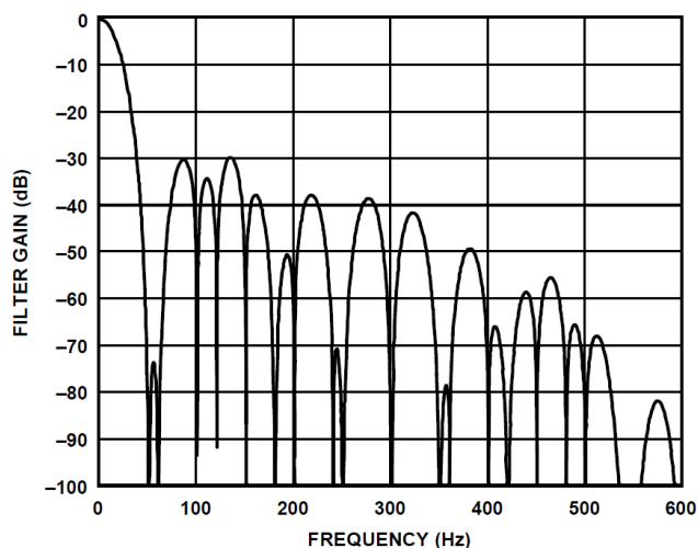
Figure 33. 20 SPS ODR, 50 ms Settling Time
