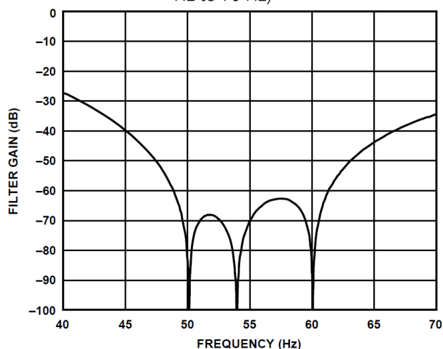
Figure 37. 25 SPS ODR, 40 ms Settling Time (40 Hz to 70 Hz)
