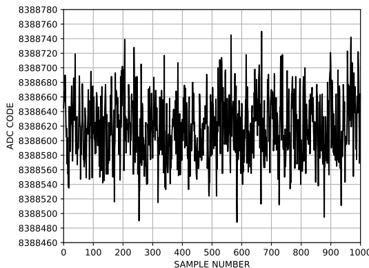
Figure 9. Noise (Output Data Rate = 31.25 kSPS)
