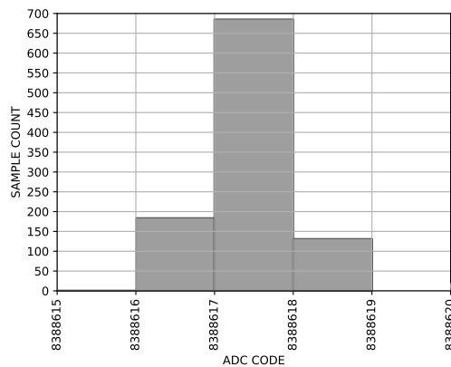
Figure 6. Histogram (Output Data Rate = 1.25 SPS)
