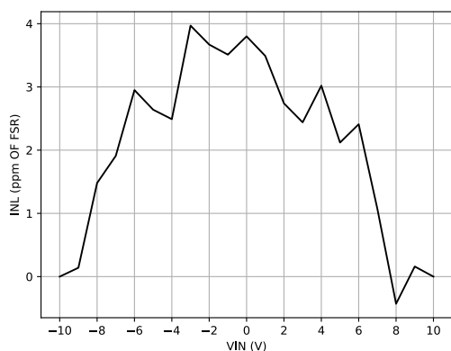
Figure 11. INL vs. VIN
