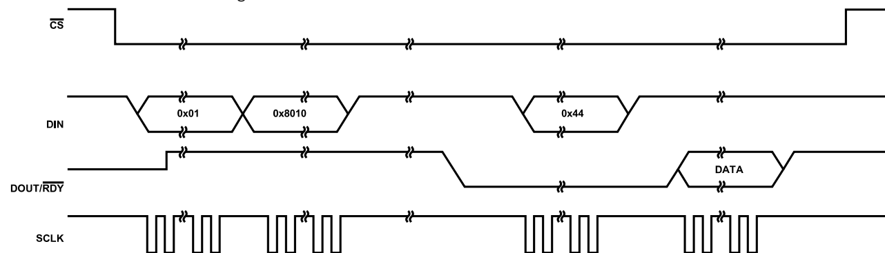
Figure 40. SPI Communication in Continuous Read Mode
