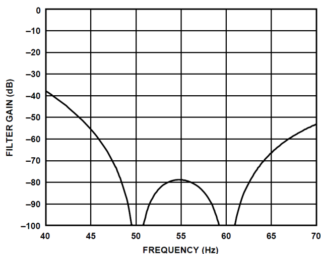
Figure 38. 16.667 SPS ODR, 60 ms Settling Time (40 Hz to 70 Hz)
