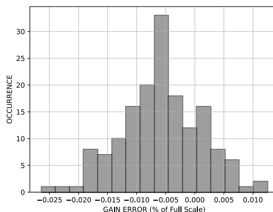
Figure 14. Gain Error Distribution Histogram
