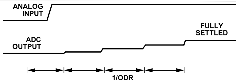
Figure 29. Step Input Without Single-Cycle Settling
