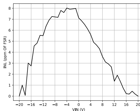
Figure 12. INL vs. VIN
