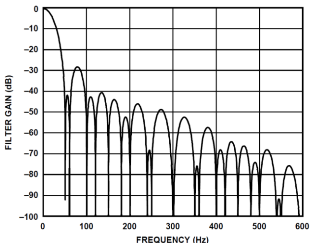
Figure 31. 27.27 SPS ODR, 36.67 ms Settling Time
