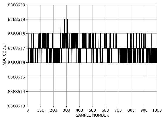
Figure 5. Noise (Output Data Rate = 1.25 SPS)
