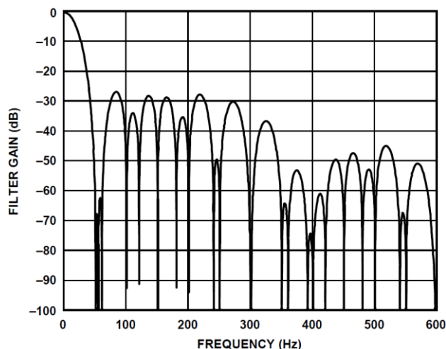
Figure 32. 25 SPS ODR, 40 ms Settling Time
