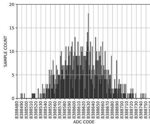
Figure 10. Histogram (Output Data Rate = 31.25 kSPS)
