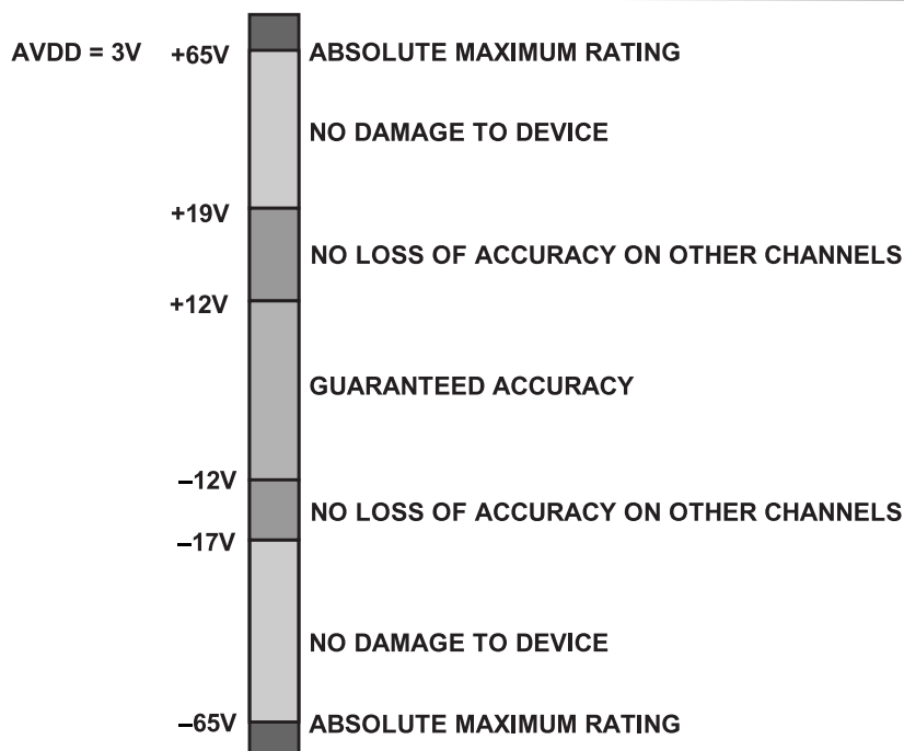
Figure 22. Absolute Input Pin Voltages, AVDD = 3 V
