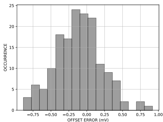
Figure 13. Offset Error Distribution Histogram
