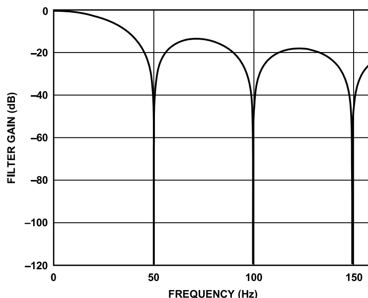
Figure 27. Sinc5 + Sinc1 Filter Response at 50 SPS ODR
