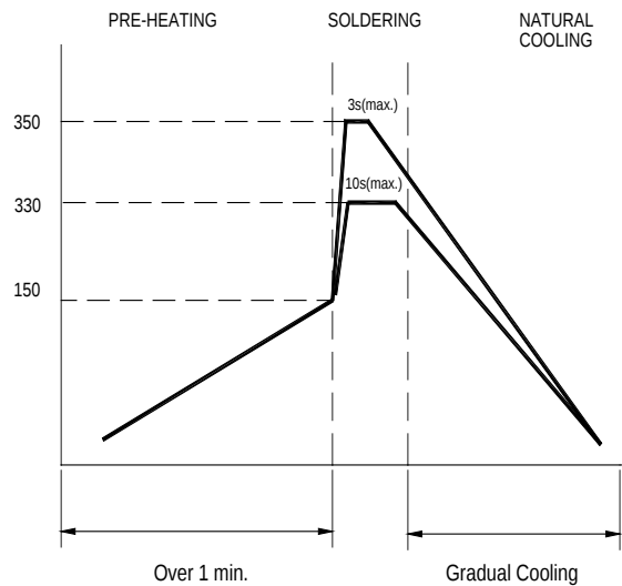
Figure 2. Hand Soldering
