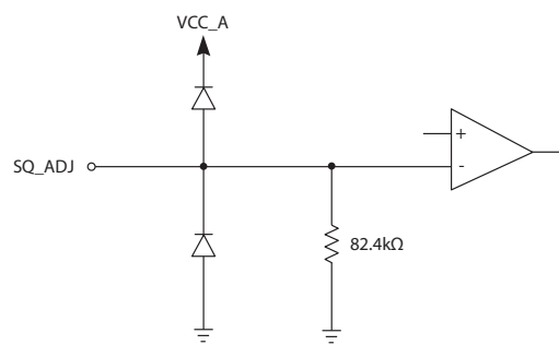
Figure 3-2: SQ_ADJ Circuit
