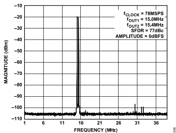
Figure 25. Dual-Tone SFDR
