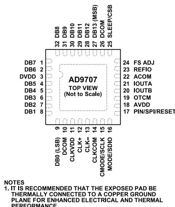
Figure 3. AD9707 Pin Configuration
