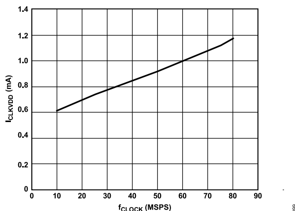
Figure 85. I_{CLKVDD} vs. f_{CLOCK} (Differential Clock Mode) at CLKVDD = 1.8\text{ V}
