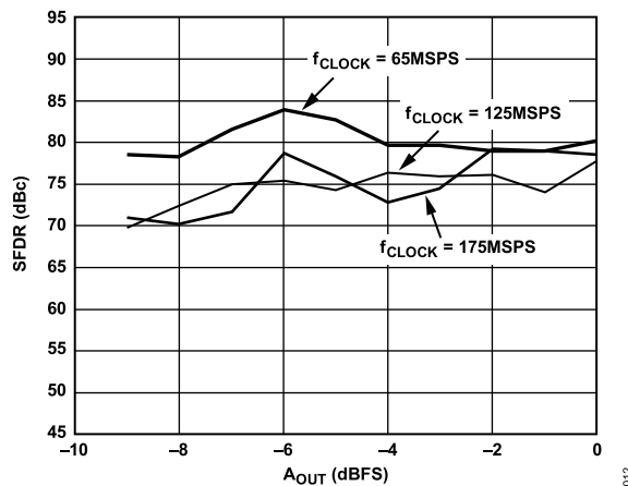
Figure 14. SFDR vs. A_{OUT} and f_{CLOCK} at f_{OUT} = f_{CLOCK}/5
