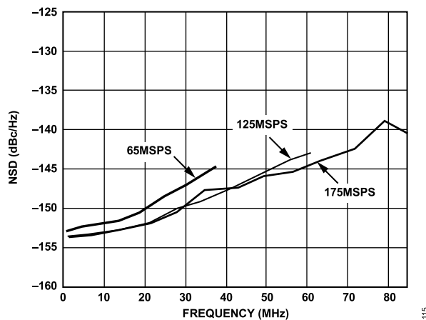
Figure 15. NSD vs. f_{OUT} and f_{CLOCK} at 0 dBFS
