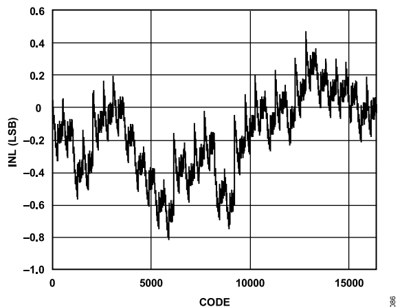
Figure 21. Typical Calibrated INL
