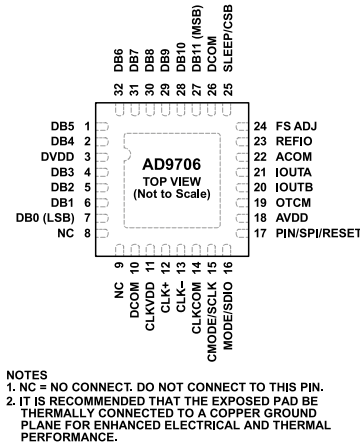
Figure 4. AD9706 Pin Configuration
