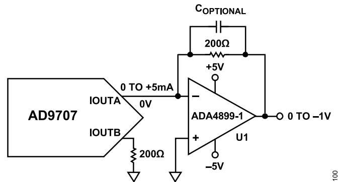
Figure 89. Unipolar Buffered Voltage
