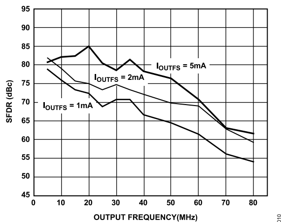
Figure 12. SFDR vs. f_{OUT} and I_{OUTFS} at 175 MSPS
