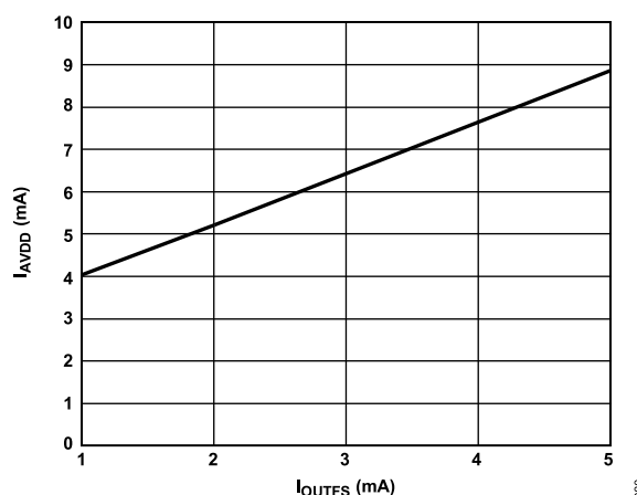
Figure 80. I_{AVDD} vs. I_{OUTFS} at AVDD = 3.3 V
