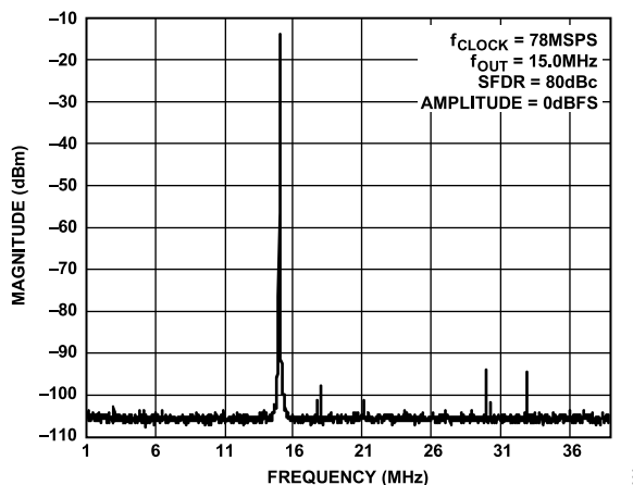
Figure 24. Single-Tone SFDR
