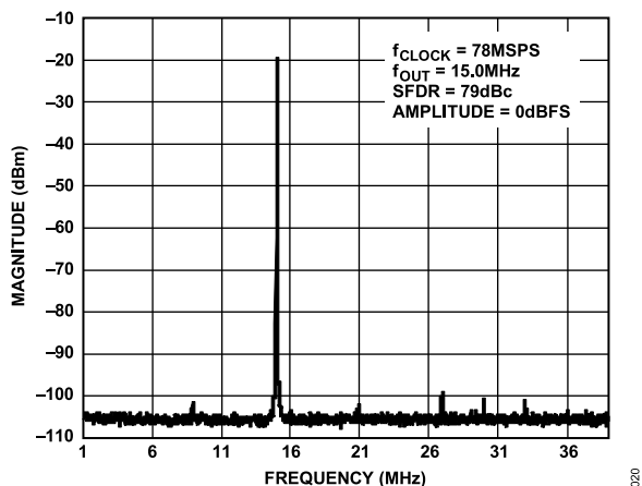
Figure 41. Single-Tone SFDR
