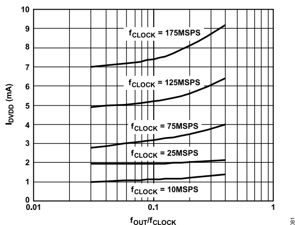
Figure 82. I_{DVDD} vs. f_{OUT}/f_{CLOCK} Ratio at DVDD = 3.3\text{ V}
