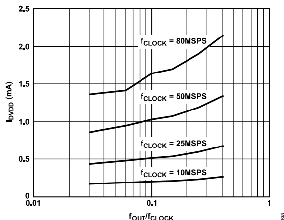
Figure 83. I_{DVDD} vs. f_{OUT}/f_{CLOCK} Ratio at DVDD = 1.8\text{ V}
