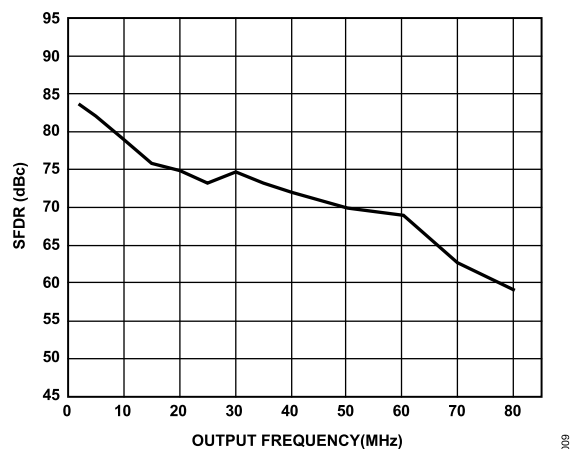
Figure 11. SFDR vs. f_{OUT} at 175 MSPS
