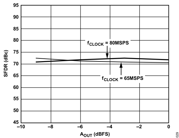
Figure 32. SFDR vs. A_{OUT} at f_{OUT} = f_{CLOCK}/5
