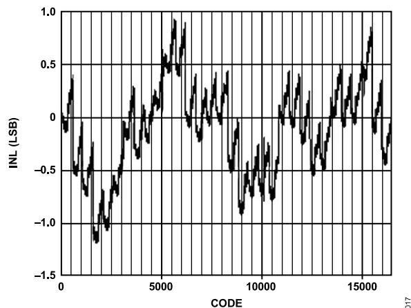
Figure 19. Typical Uncalibrated INL
