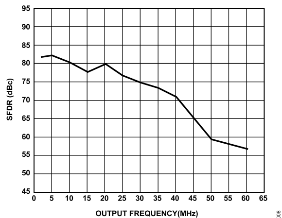
Figure 10. SFDR vs. f_{OUT} at 125 MSPS
