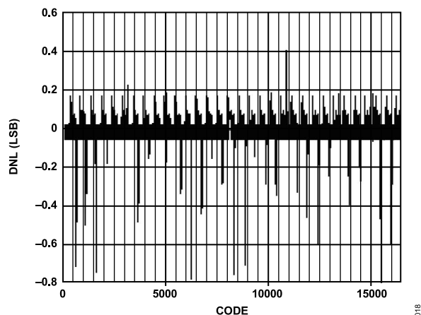
Figure 20. Typical Uncalibrated DNL
