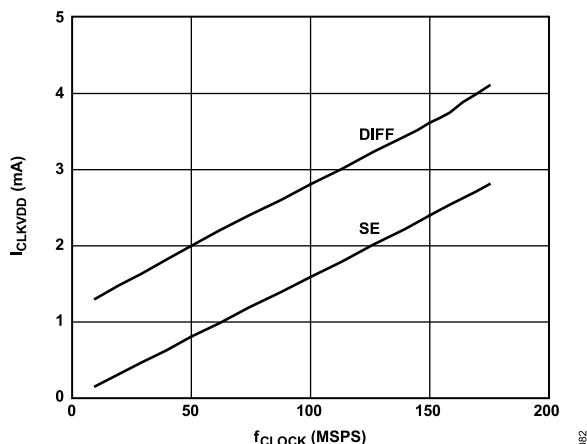
Figure 84. I_{CLKVDD} vs. f_{CLOCK} at CLKVDD = 3.3\text{ V}
