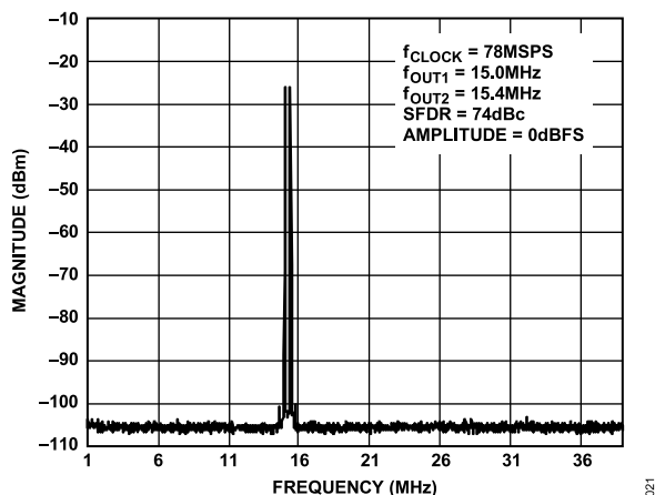
Figure 42. Dual-Tone SFDR
