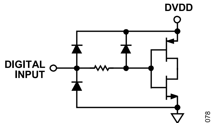
Figure 79. Equivalent Digital Input
