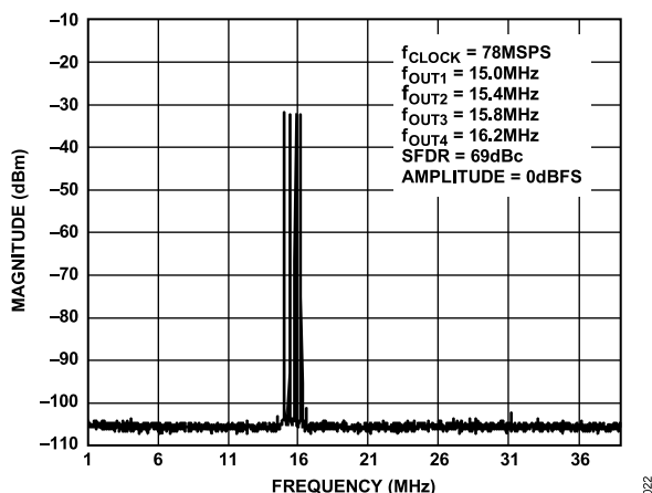
Figure 43. Four-Tone SFDR
