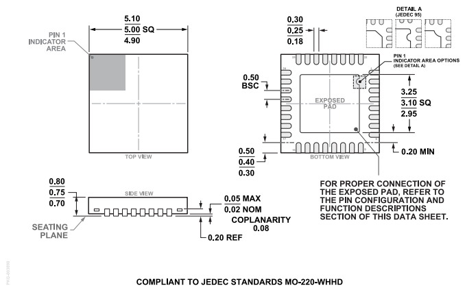
Figure 91. 32-Lead Lead Frame Chip Scale Package [LFCSP] 5 mm × 5 mm Body and 0.75 mm Package Height (CP-32-7) Dimensions shown in millimeters
