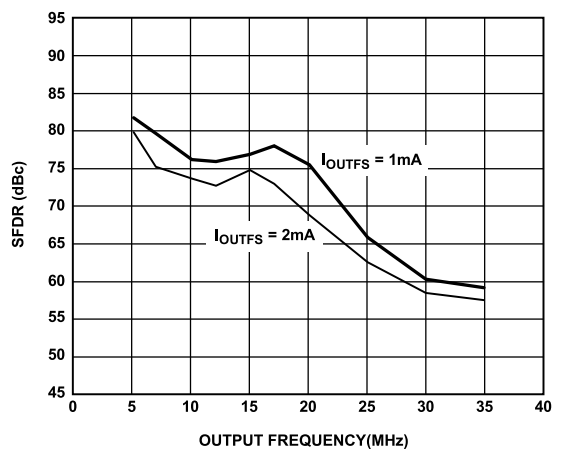
Figure 31. SFDR vs. f_{OUT} and I_{OUTFS} at 80 MSPS
