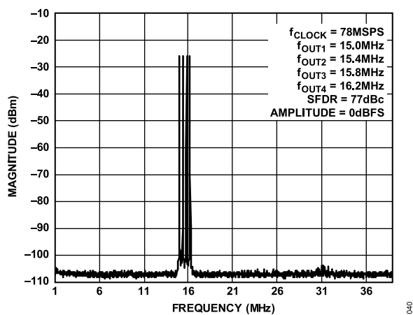
Figure 26. Four-Tone SFDR
