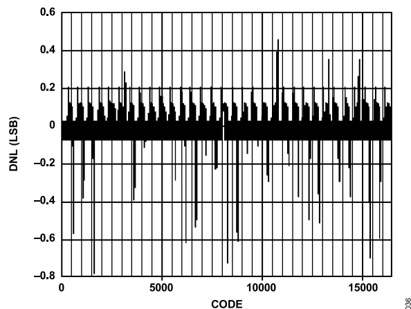
Figure 39. Typical Uncalibrated DNL
