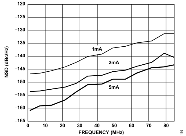
Figure 16. NSD vs. f_{OUT} and I_{OUTFS} at 175 MSPS
