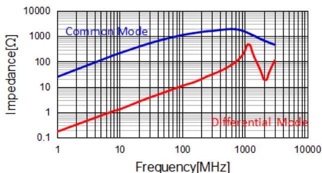
WBA1206D-102PT-HF
