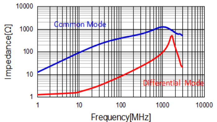
WBA1206D-361PT-HF
