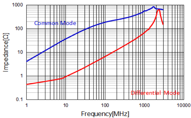
WBA1206D-261PT-HF
