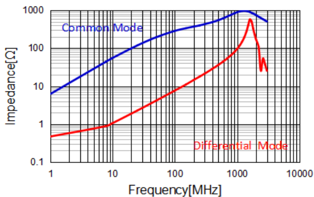
WBA1206D-261PT-HF
