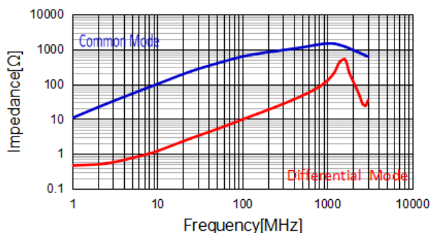
WBA1206D-601PT-HF
