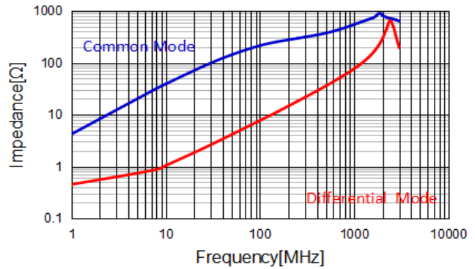
WBA1206D-361PT-HF
