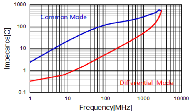
WBA1206D-121PT-HF
