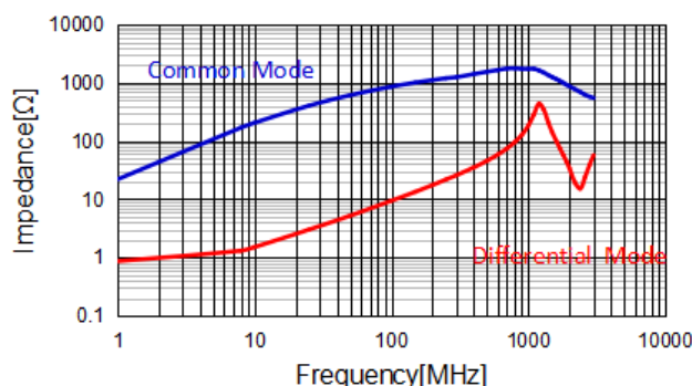
WBA1206D-801PT-HF
