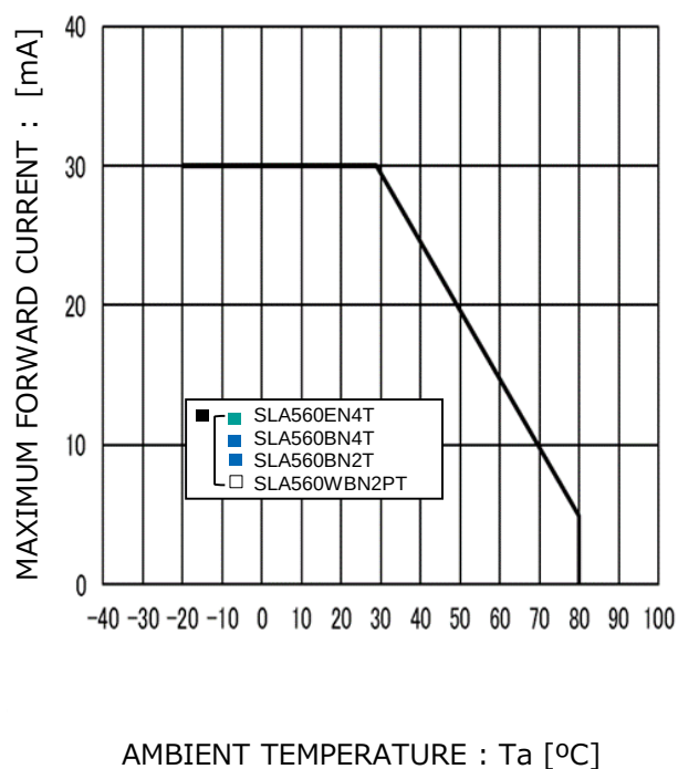
Fig.4 Derating
