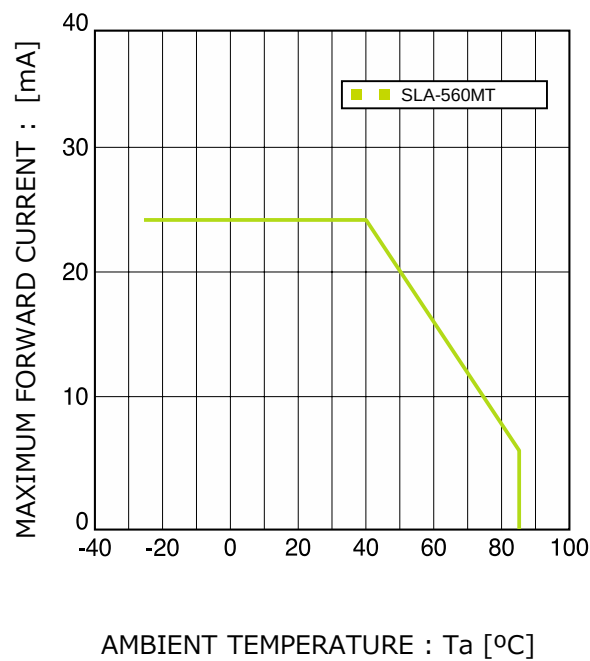
Fig.4 Derating
