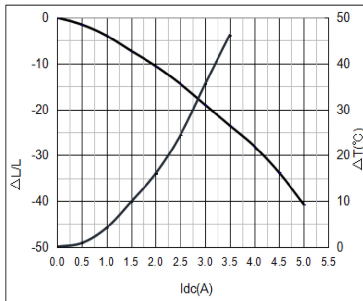
3R3 DC Bias & Temperature Characteristics
