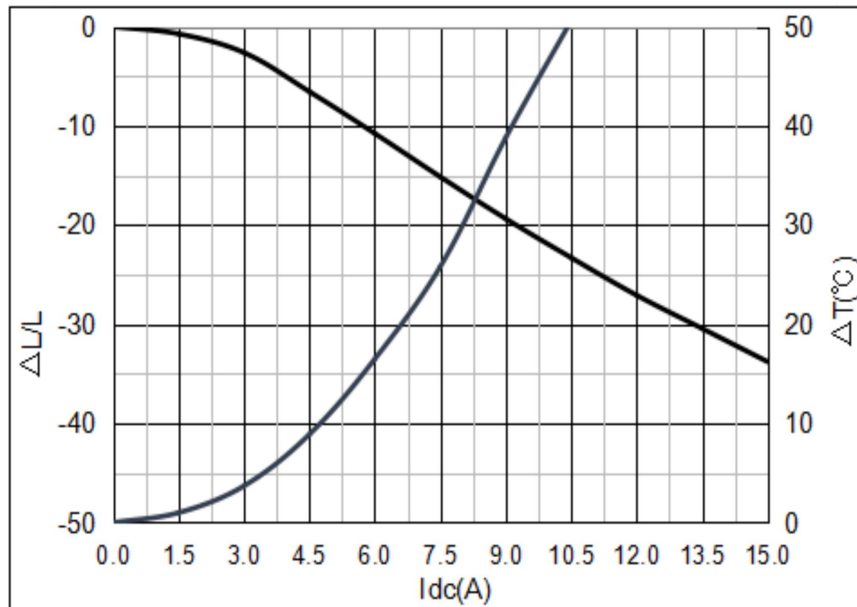
6R8 DC Bias & Temperature Characteristics
