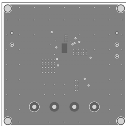
Figure3 – Inner Layer 1
