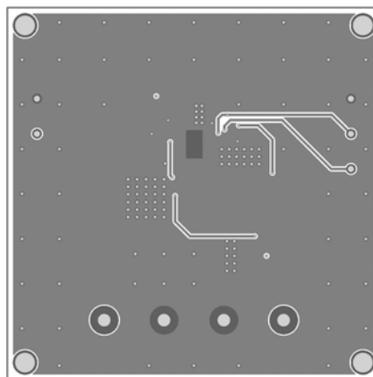
Figure 4 – Inner Layer 2
