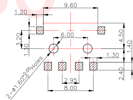
P.C.B.MOUNTING DETAIL
