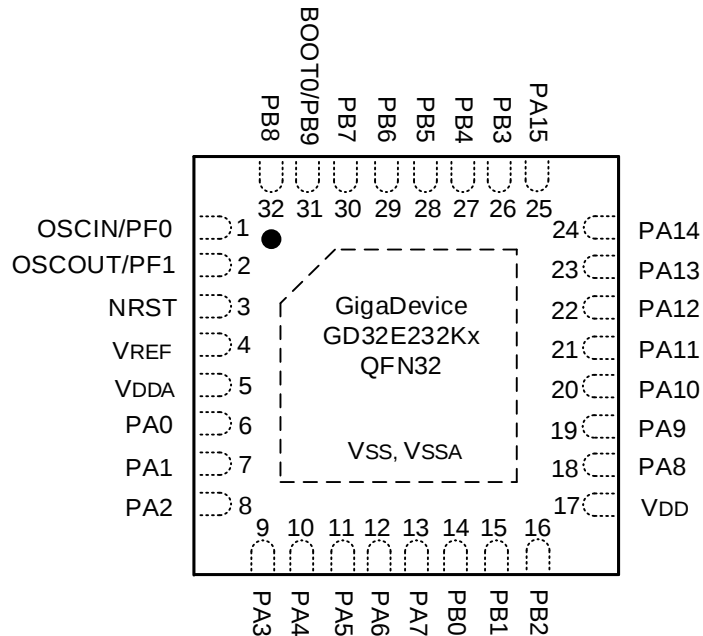
Figure 2-2. GD32E232Kx QFN32 pinouts
