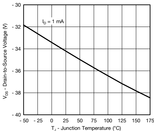
BVDSS vs. Junction Temperature
