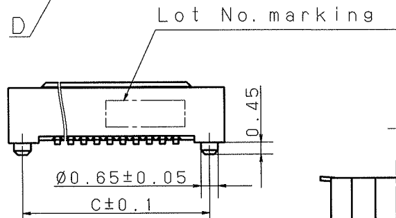
Setting drawing
