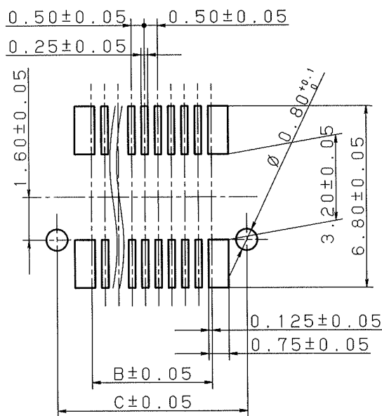
Recommended PC board pattern (mounting pad layout) (TOP VIEW)
