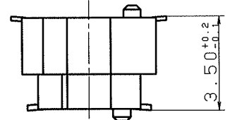
AXK600200Y header used
