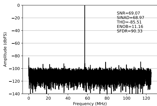
(c) 输入信号频率 = 57MHz
