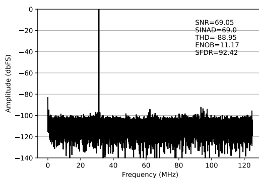
(b) 输入信号频率 = 31MHz
