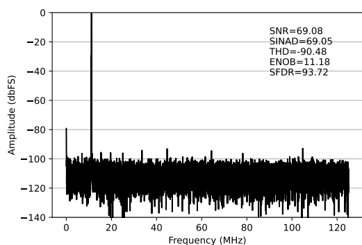
(a) 输入信号频率 = 11MHz
