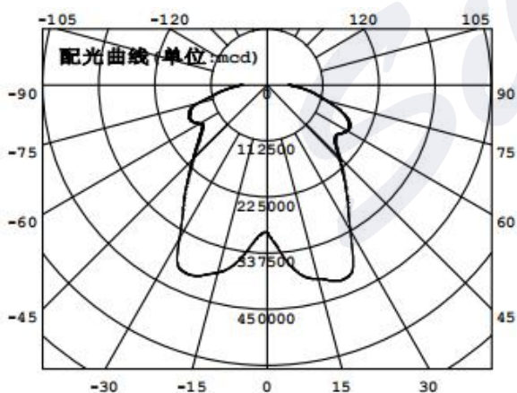
Luminous angle
