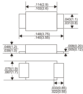
SOD123FL
