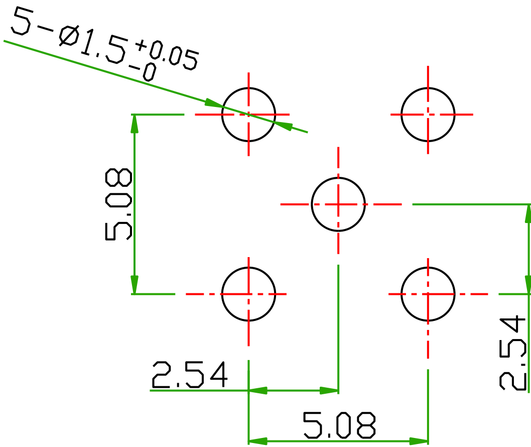
PCB LAYOUT
