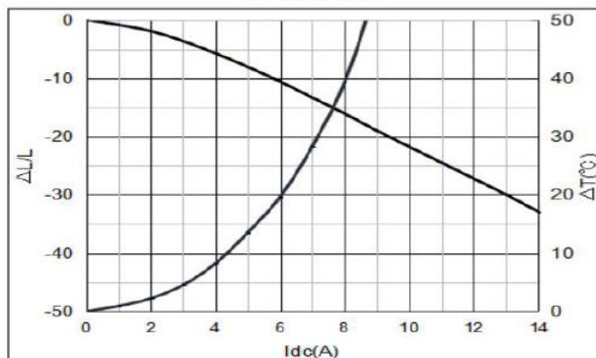
YSPI0850-100M
