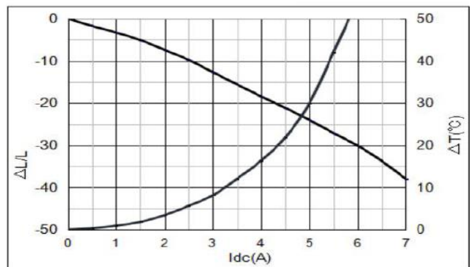
YSPI0850-150M
