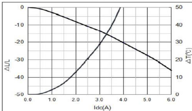
YSPI0850-680M
