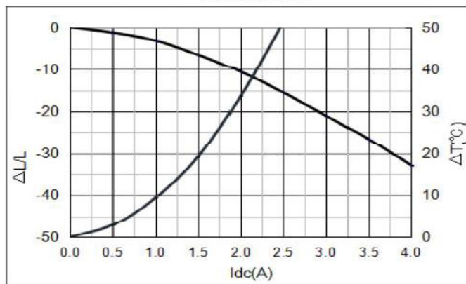
YSPI0850-680M
