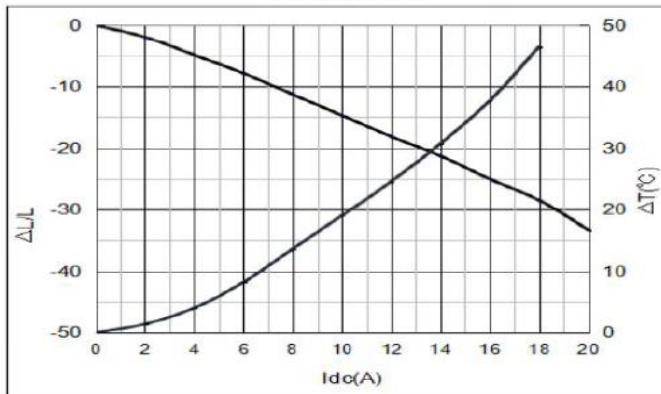
YSPI0850-2R2M
