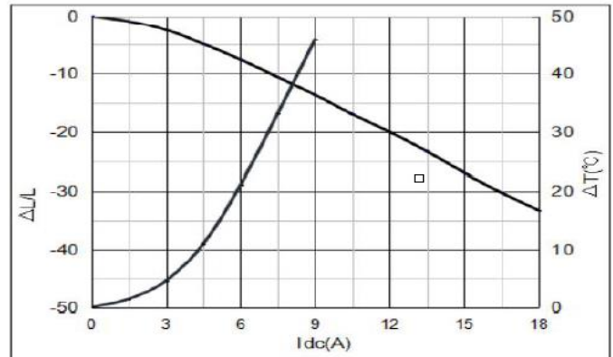
YSPI0850-6R8M
