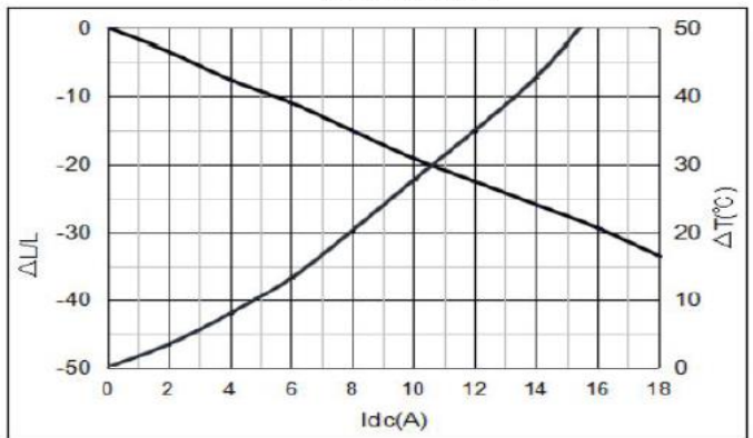
YSPI0850-3R3M
