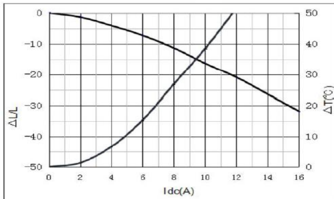
YSPI0850-4R7M
