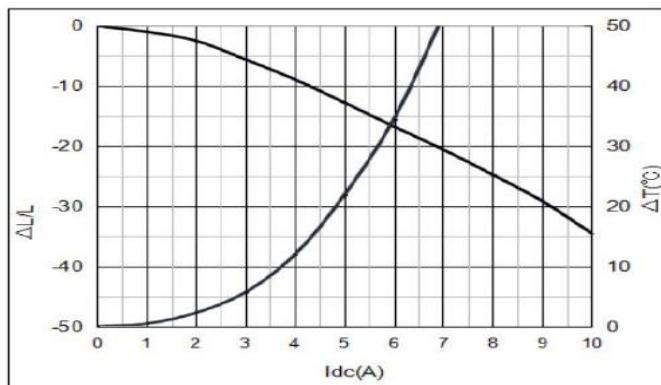
YSPI0850-100M
