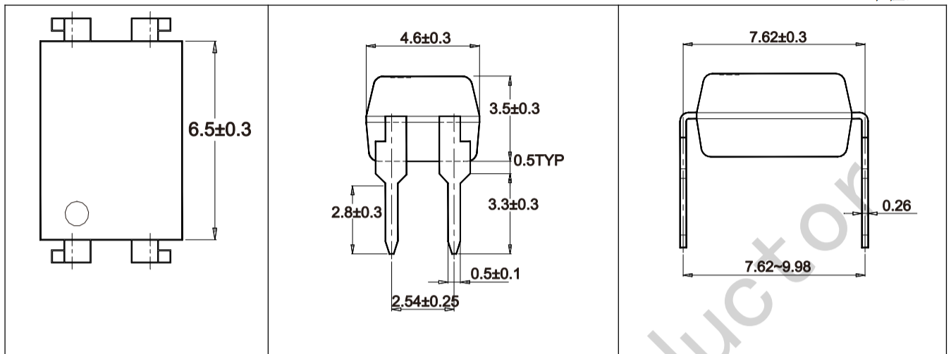
4-pin DIP
