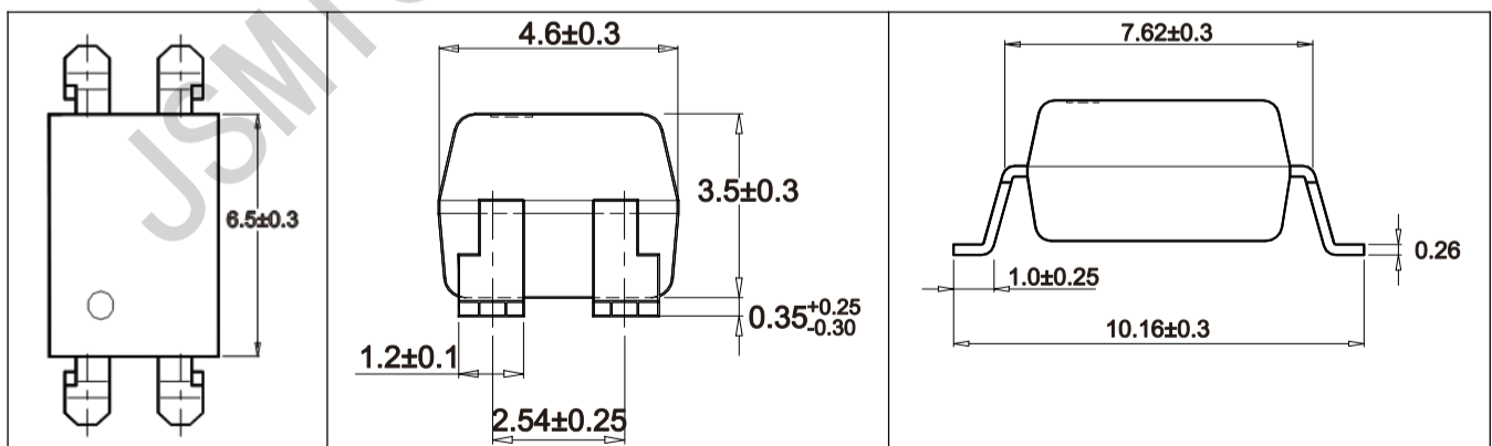
4-pin SMD
