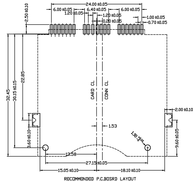
RECOMMENDED P.C.B. BOARD LAYOUT
