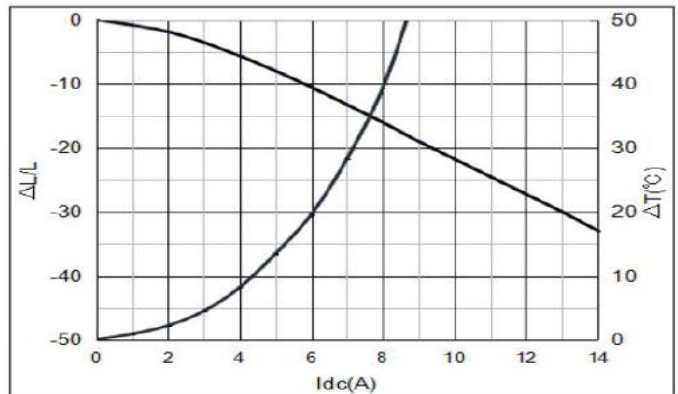
YSPI0850-100M
