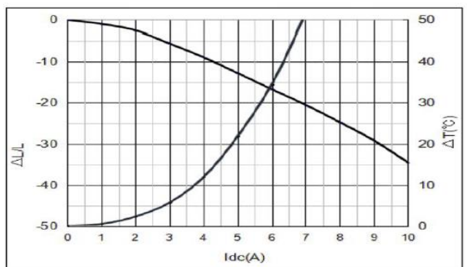
YSPI0850-100M
