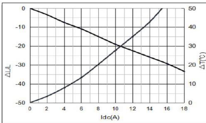
YSPI0850-3R3M
