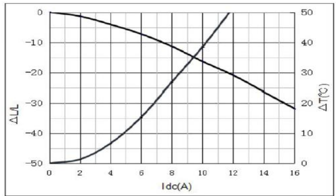
YSPI0850-4R7M
