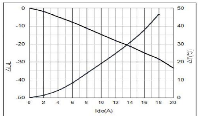
YSPI0850-2R2M
