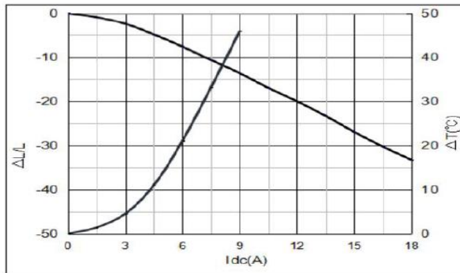
YSPI0850-6R8M
